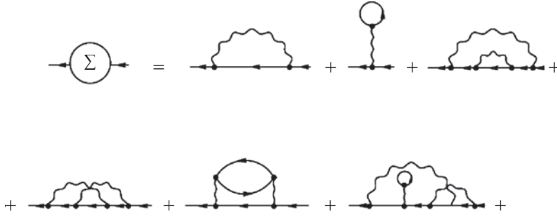
Figure 11.7. Simplest diagrams for irreducible self-energy part.
