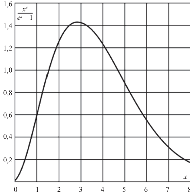
Figure 4.2. Planck function \frac{x^3}{e^x - 1} ; x = \frac{\hbar\omega}{T} .
