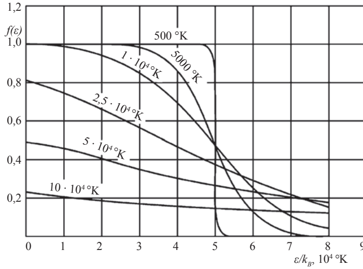
Figure 4.1. Fermi distribution function for different temperatures for \varepsilon_F/k_B = 50\,000\text{ K} .
