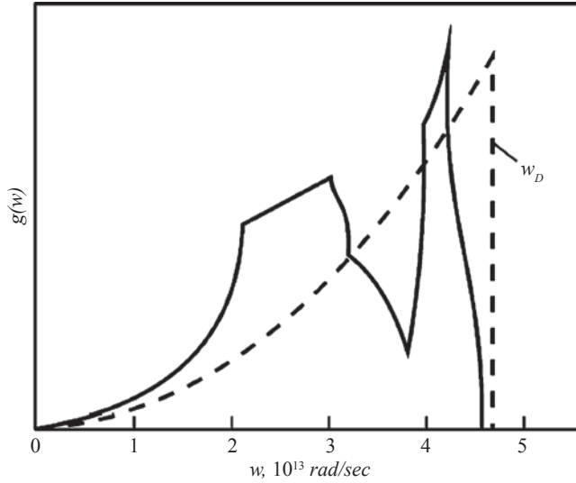
Figure 5.1. Phonon density of states in copper determined from neutron scattering experiments. The dashed line corresponds to the Debye model which is fixed by demanding equality of the areas under this line and the experimental density of states. Debye temperature \theta_D = 340 K.
