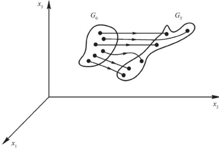
Figure 1.1. The change of initial volume G_0 in the phase space due to the motion of phase points representing an ensemble according to the Liouville theorem.
